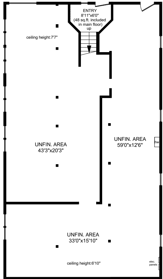
LOWER FLOOR 2019 SQ.FT
